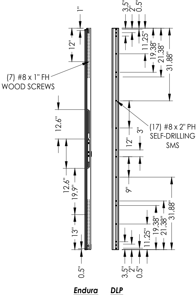
ASTRAGAL SCREW LOCATIONS
