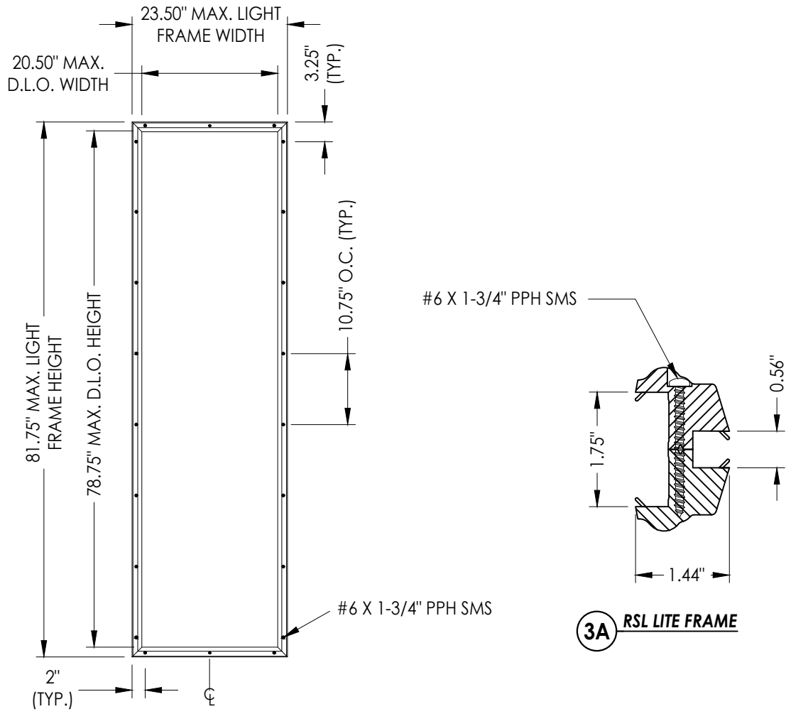
RSL LITE FRAME
